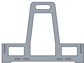
Spine x1 Part KC22-01
